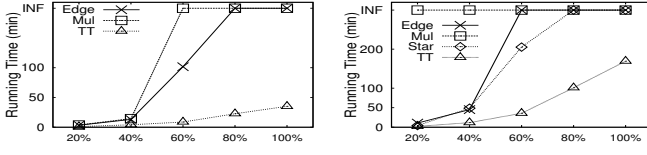
(a) Query q_1 on fs (b) Query q_4 on fs
