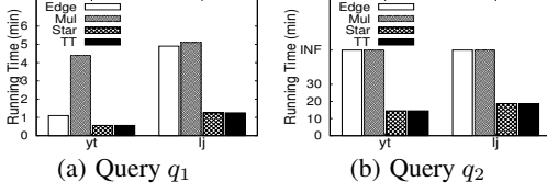
Figure 6: Vary Algorithms
