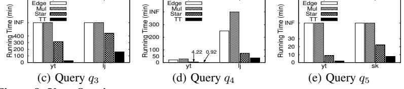
Figure 8: Vary Queries
